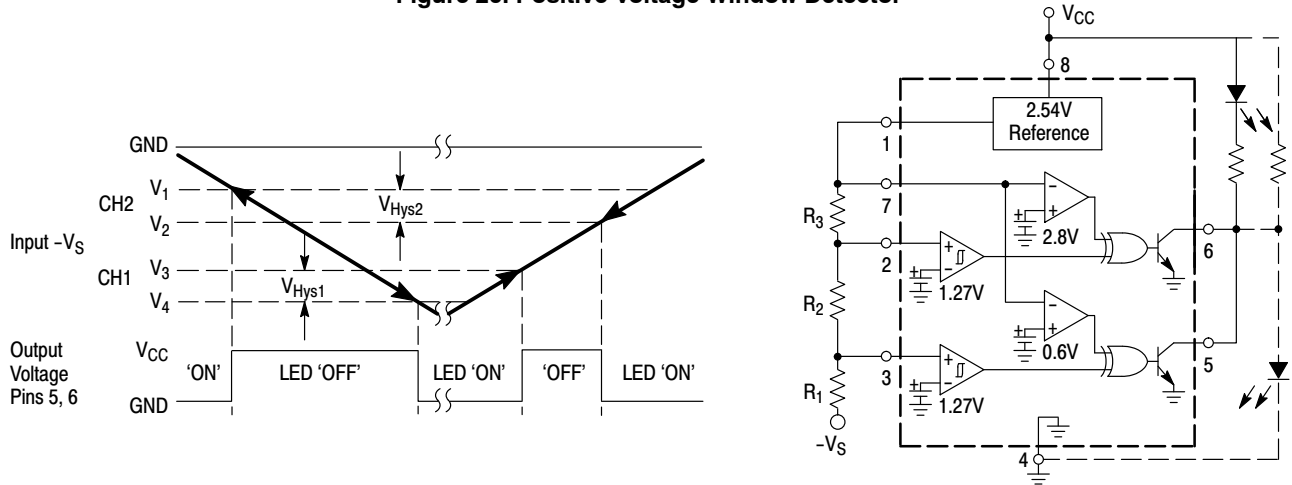
Figure 20. Positive Voltage Window Detector
