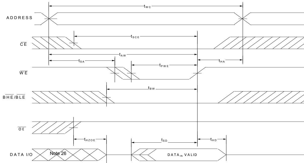
Figure 9. Write Cycle No. 3 ( \overline{WE} Controlled) [24, 25]
