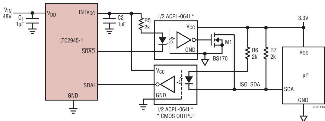
Figure 13. Opto-Isolation of a 10kHz I²C Interface Between LTC2945 and Microcontroller (SCL Omitted for Clarity)
