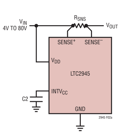
Figure 2a. LTC2945 Derives Power from the Supply Being Monitored
