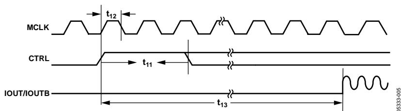
Figure 5. CTRL Timing
