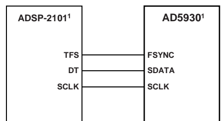
Figure 36. ADSP-2101 to AD5930 Interface
