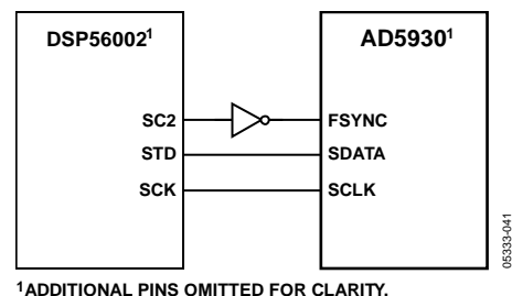
Figure 39. DSP56002 to AD5930 Interface
