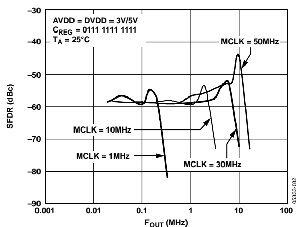
Figure 14. Wideband SFDR vs. F_{OUT} for Various MCLK Frequencies
