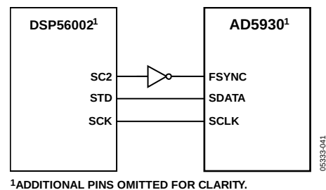
Figure 39. DSP56002 to AD5930 Interface
