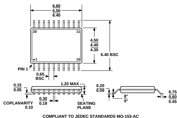
Figure 42. 20-Lead Thin Shrink Small Outline Package (TSSOP) (RU-20)
