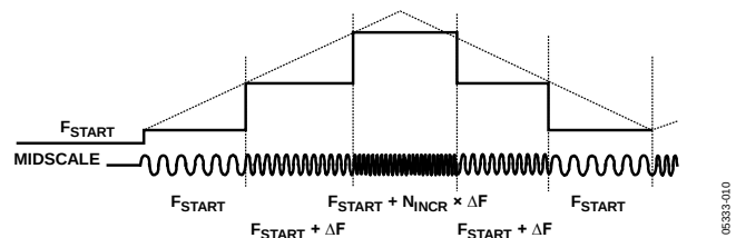
Figure 32. Triangular-Sweep Profile
