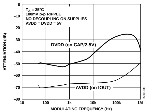
Figure 20. PSSR
