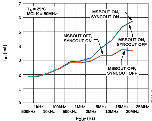
Figure 10. I_{DD} vs. F_{OUT} for Various Digital Output Conditions
