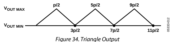
Figure 34. Triangle Output
