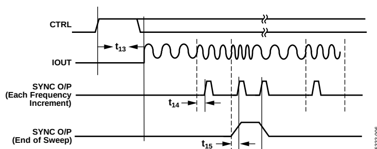
Figure 6. CTRL Timing, Saw-Sweep Mode
