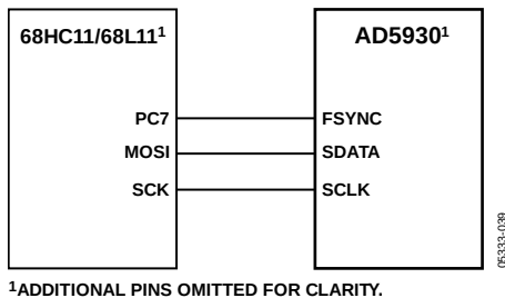
Figure 37. 68HC11/68L11 to AD5930 Interface
