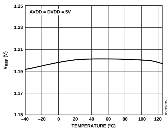
Figure 16. V_{REF} vs. Temperature
