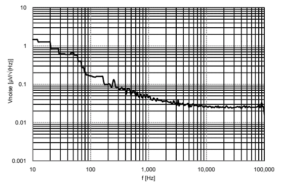
Figure 17. Noise spectral density (V OUT = 3.0 V; I OUT = 10 mA)
