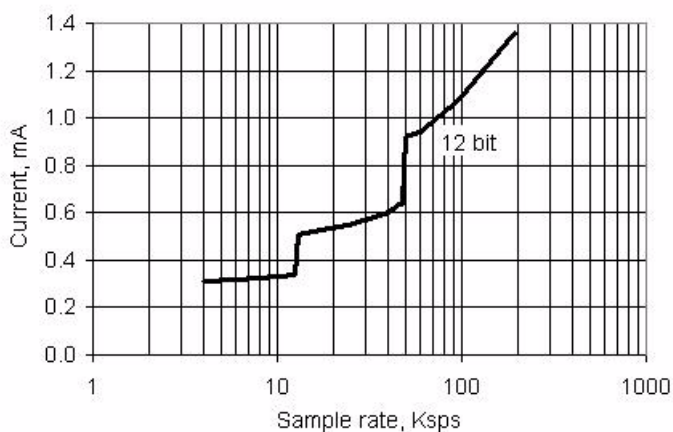
Figure 11-23. Delta-sigma ADC IDD vs sps, Range = \pm 1.024 V, Continuous Sample Mode, Input Buffer Bypassed
