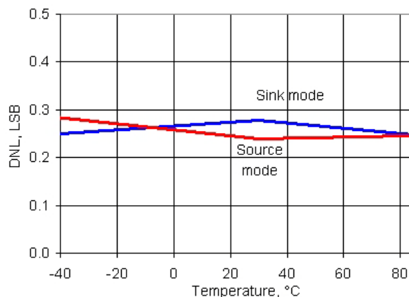
Figure 11-29. IDAC DNL vs Temperature, Range = 255 \mu A, High speed mode
