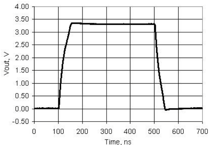
Figure 11-19. SIO Output Rise and Fall Times, Slow Strong Mode, V DDIO = 3.3 V, 25 pF Load
