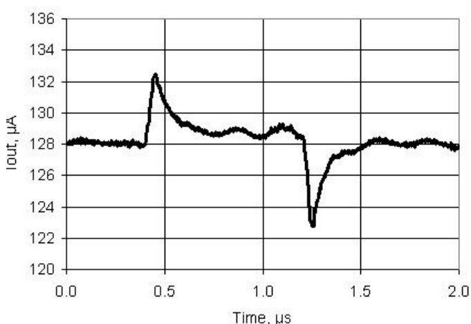
Figure 11-37. IDAC Current Noise, 255 \mu A Mode, Source Mode, High speed mode, V_{DDA} = 5 V
