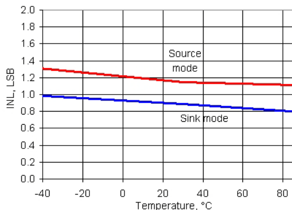
Figure 11-28. IDAC INL vs Temperature, Range = 255 \mu A, High speed mode
