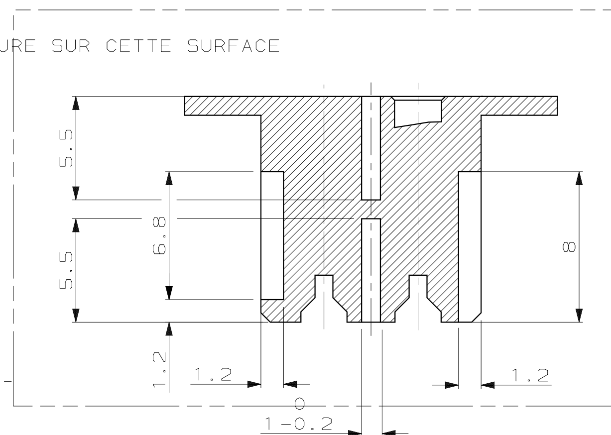
SECTION CC
