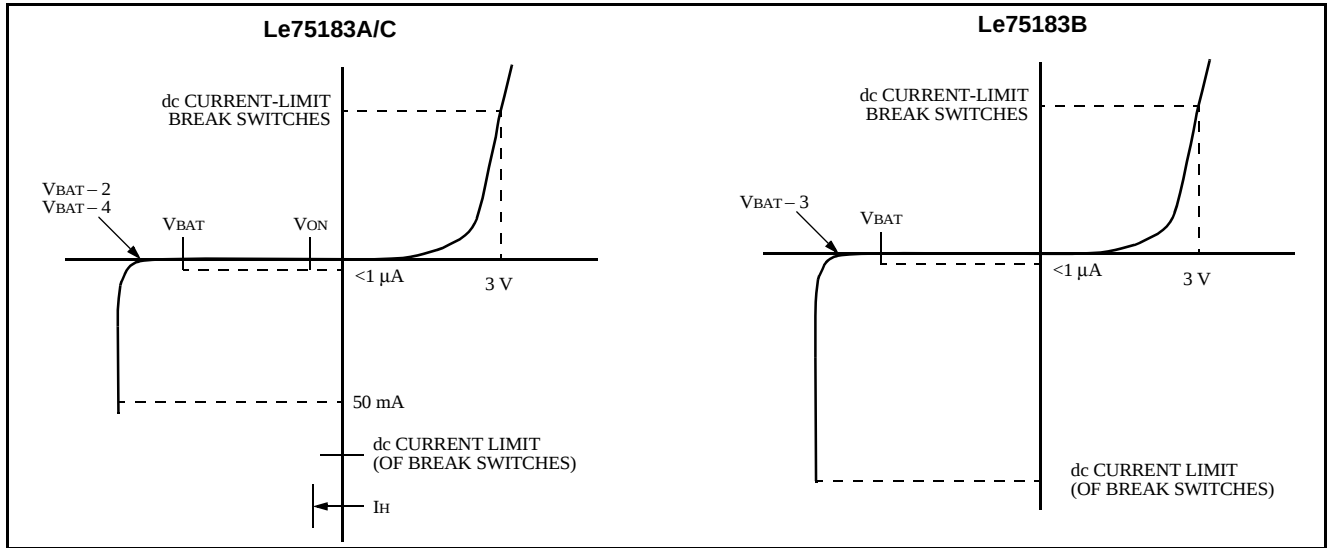
Figure 3 - Protection Circuits
