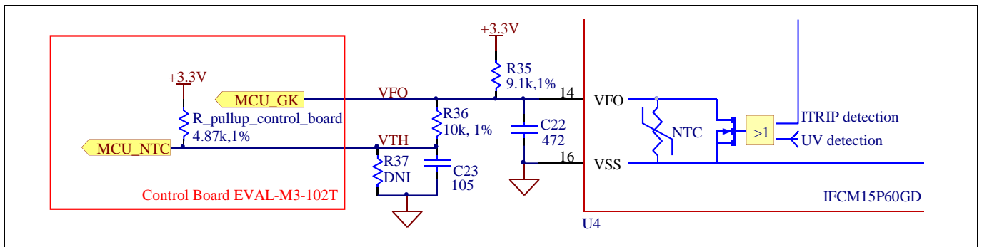
Figure 27 Overtemperature protection circuit schematic for Eval-M3-CM615PN and Eval-M3-102T
