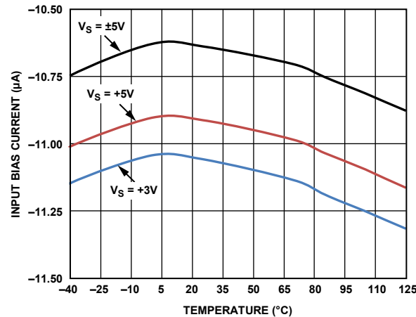
Figure 38. Input Bias Current vs. Temperature for Various Supplies
