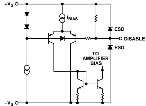
Figure 45. DISABLE Circuit
