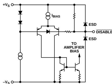
Figure 45. \overline{\text{DISABLE}} Circuit
