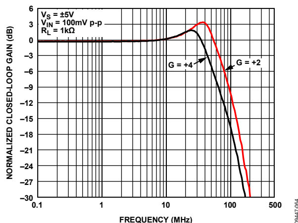
Figure 53. Frequency Response of V_{02}/V_{IN}
