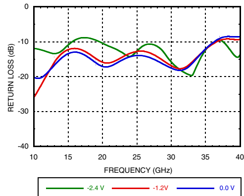
Input Return Loss, Vctrl1 = Vctrl2
