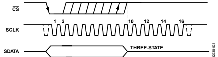
Figure 21. Entering Power-Down Mode
