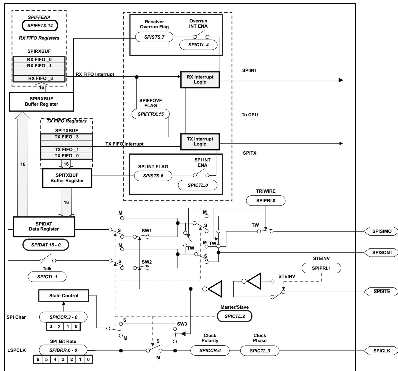
Figure 6-14. SPI Module Block Diagram (Slave Mode)
