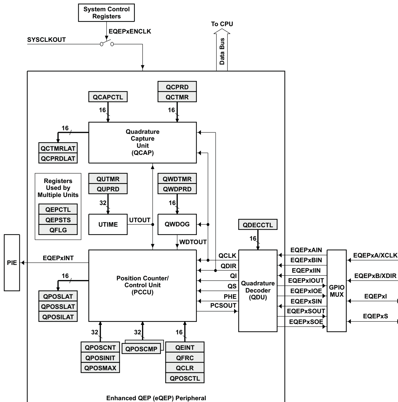
Figure 6-27. eQEP Functional Block Diagram
