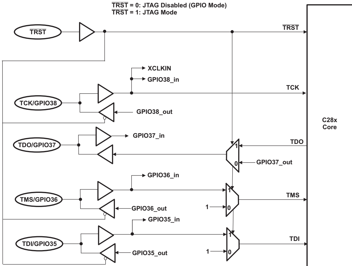
Figure 6-28. JTAG/GPIO Multiplexing
