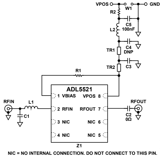
NIC = NO INTERNAL CONNECTION. DO NOT CONNECT TO THIS PIN. Figure 54. Evaluation Board Schematic
