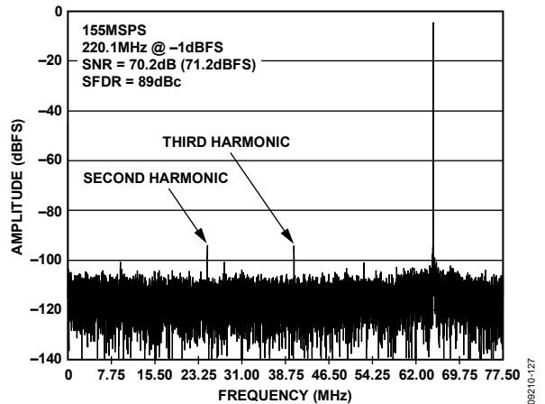
Figure 28. AD9641-155 Single-Tone FFT with f_{IN} = 220.1 MHz
