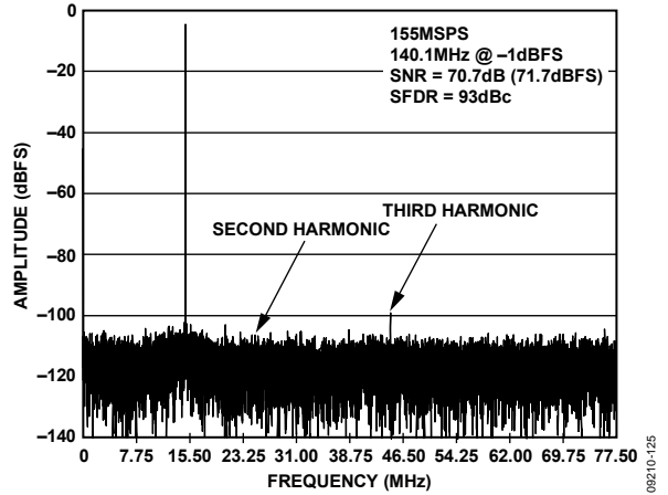
Figure 26. AD9641-155 Single-Tone FFT with f_{IN} = 140.1 MHz
