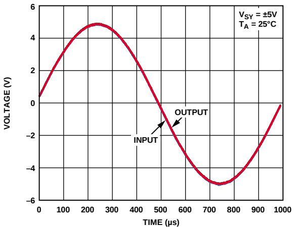
Figure 58. No Phase Reversal
