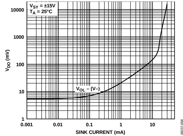
Figure 71. Dropout Voltage vs. Sink Current
