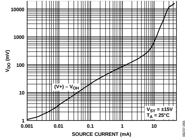
Figure 70. Dropout Voltage vs. Source Current
