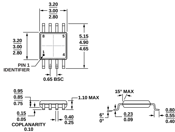
Figure 98. 8-Lead Mini Small Outline Package [MSOP] (RM-8) Dimensions shown in millimeters
