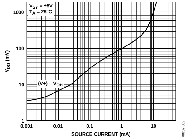
Figure 42. Dropout Voltage vs. Source Current
