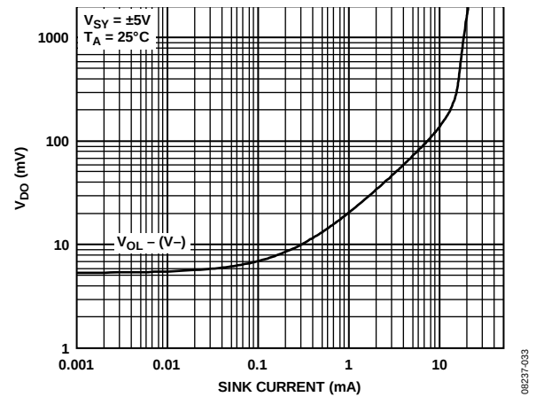
Figure 43. Dropout Voltage vs. Sink Current
