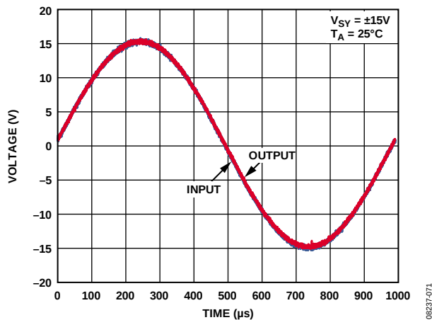
Figure 86. No Phase Reversal
