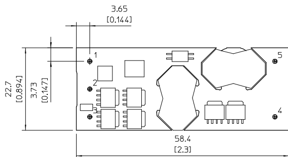
RECOMMENDED FOOTPRINT - TOP VIEW
