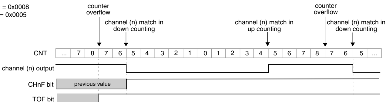
Figure 27-47. CPWM signal with ELSnB:ELSnA = X:1
