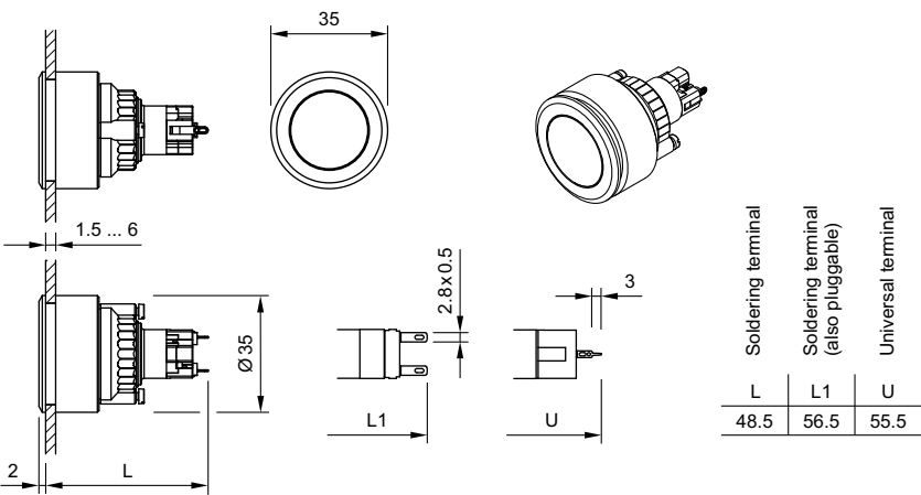
24 Indicator actuator, flush mounting page 13
