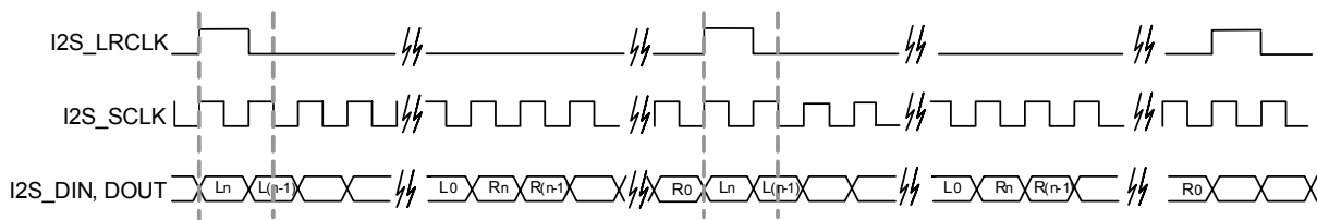
Figure 13. PCM Formats
