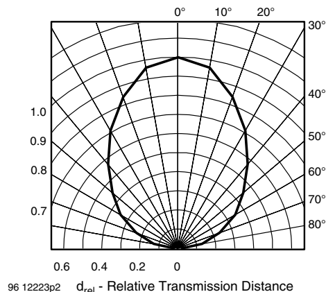
Fig. 4 - Horizontal Directivity
