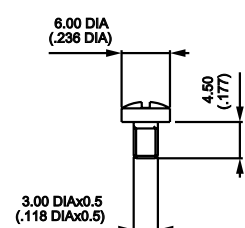
CONNECTING SCREW U03
