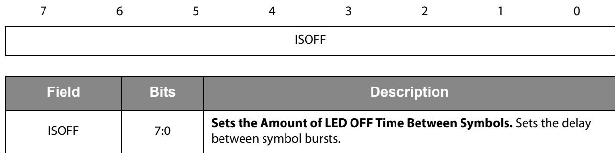
Figure 67: Configuration Register A3
