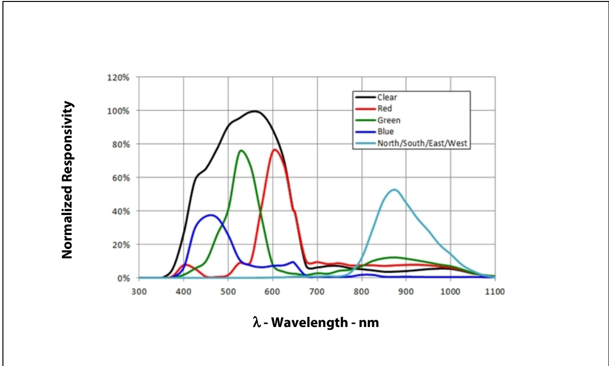
Figure 18: Spectral Responsivity
