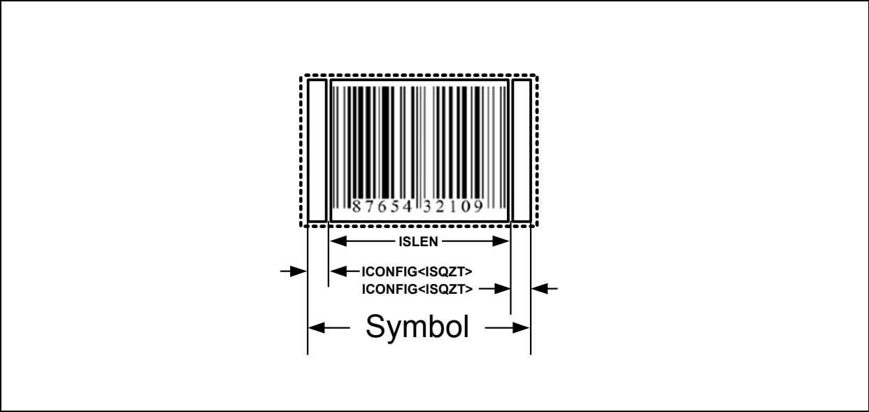
Figure 41: IRBeam Symbol
