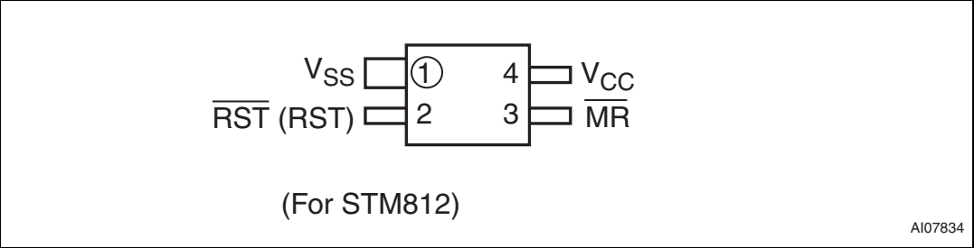
Figure 4. SOT143-4 connections
