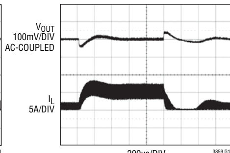
Load Step (Boost) Pulse-Skipping Mode
