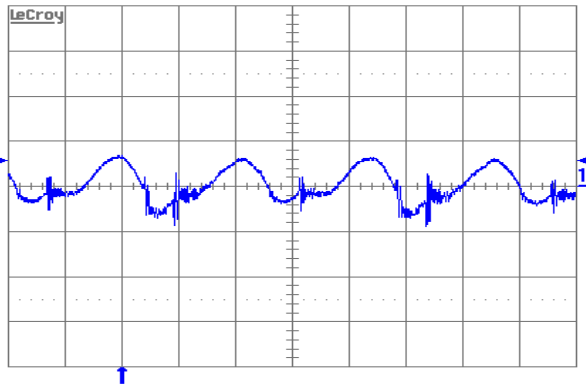
Figure 10. Output voltage ripple (20 mV/div.) at full rated load current into a resistive load with C_o = 10\mu\text{F tantalum} + 1\mu\text{F slew rate: } 5\text{ A}/\mu\text{s} . C_o = 470\mu\text{F POS} + 1\mu\text{F cer. ceramic} and V_{in} = 48\text{ V} . Time scale: 1 \mu\text{s}/\text{div} . Time scale: 0.2ms/div.
