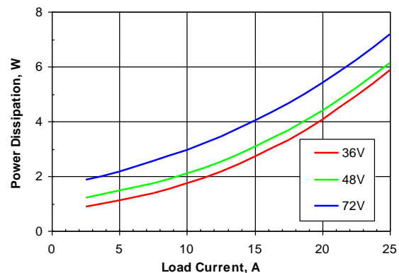
Figure 4. Power dissipation vs. load current and input voltage for SSQE48T25012 converter mounted vertically with air flowing from pin 1 to pin 3 at a rate of 300 LFM (1.5 m/s) and T_a = 25^\circ\text{C} .
