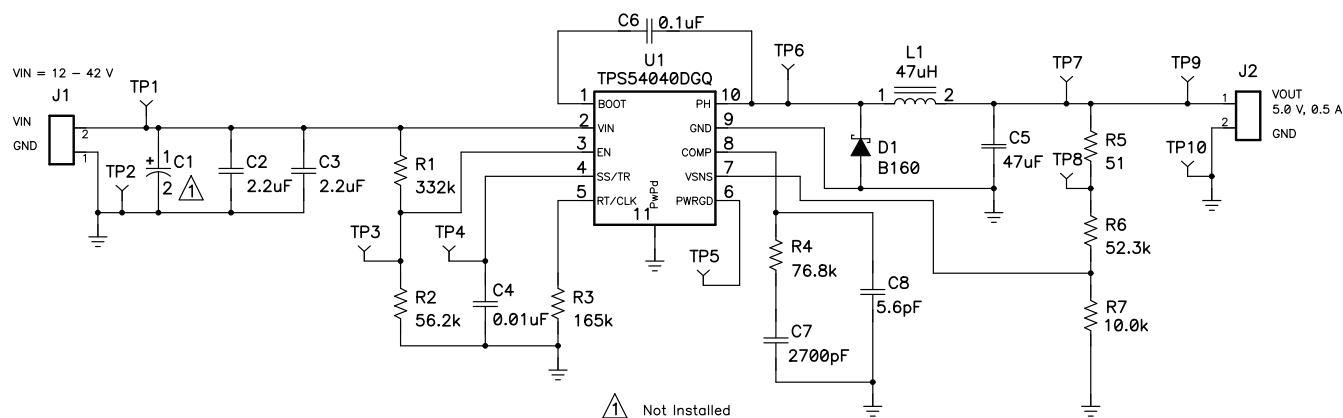
Figure 14. TPS54040EVM-456 Schematic
