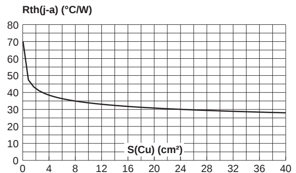
Fig. 10: Thermal resistance junction to ambient versus copper surface under tab (Epoxy printed circuit board FR4, copper thickness : 35\text{ }\mu\text{m} ). (STPS10L25G only)
