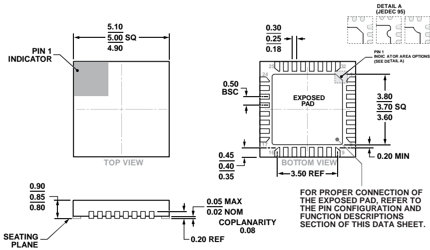
COMPLIANT TO JEDEC STANDARDS MO-220-VHHD-4. Figure 18. 32-Lead Lead Frame Chip Scale Package [LFCSP] 5 mm x 5 mm Body and 0.85 mm Package Height (HCP-32-1) Dimensions shown in millimeters
