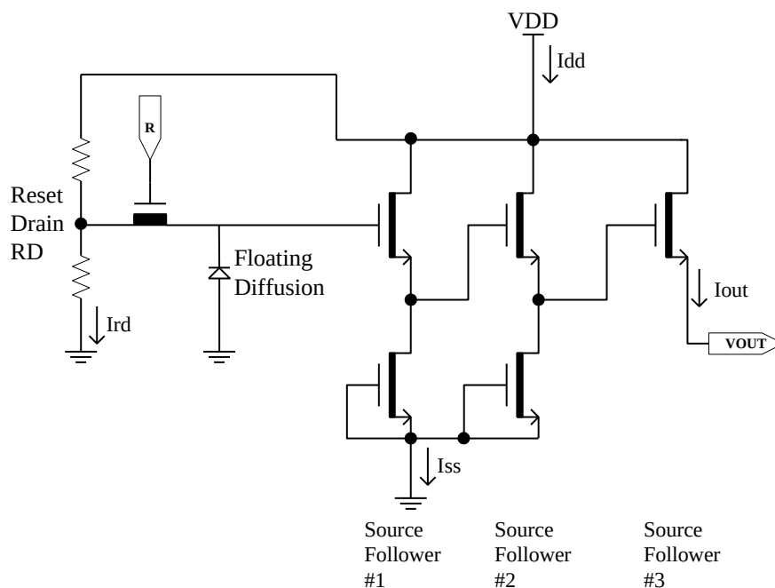
Figure 12: Output Amplifier
