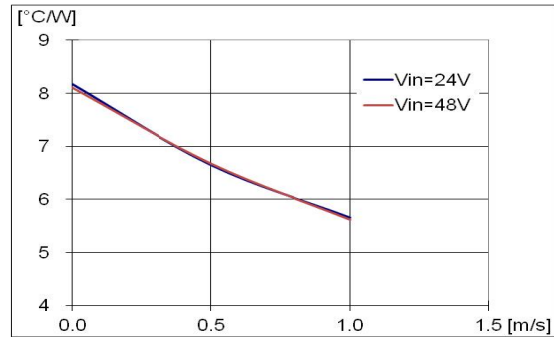
Figure 15. Thermal Resistance for the Open Frame Module; Airflow in the Transverse Direction from V_{out(-)} to V_{out(+)} ; V_{IN} = 24\text{V} or 48\text{V} , V_O=3.3\text{V} .
