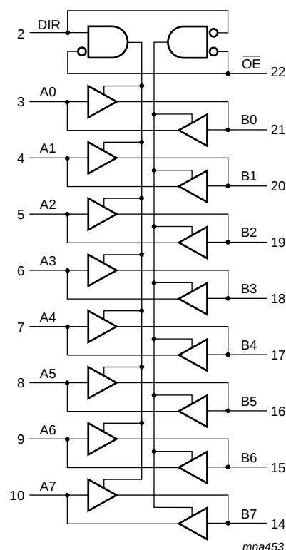
Fig 2. Logic diagram
