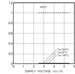
Fig.38 Input leak current ILI(CS,SK,DI)
