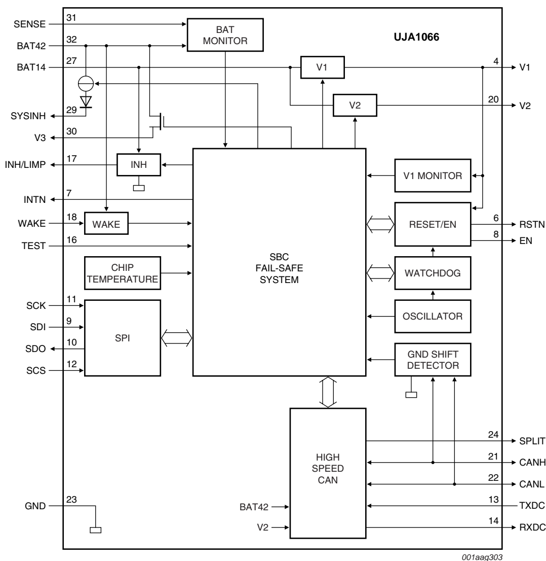
Fig 1. Block diagram
