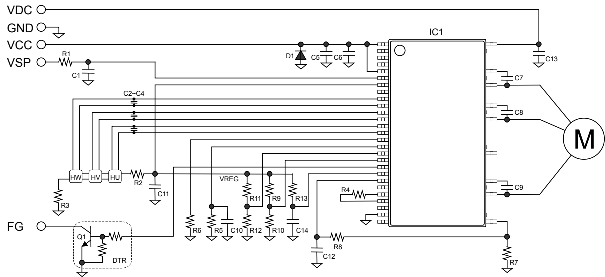
Figure 47. Application Example (150° Commutation Driver)
