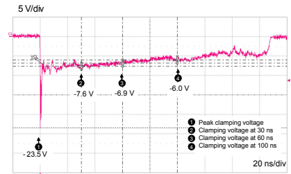
Figure 5. ESD response to IEC 61000-4-2 (-8 kV contact discharge)
