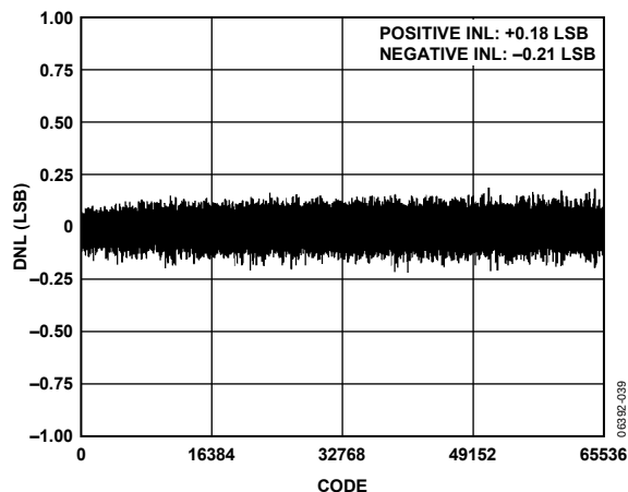
Figure 9. Differential Nonlinearity vs. Code, REF = 5 V
