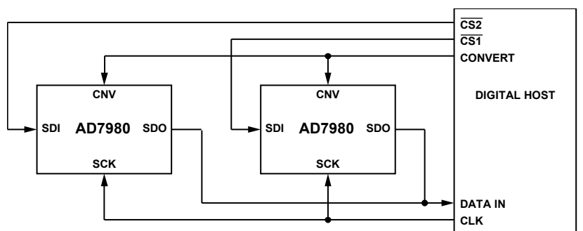
Figure 35. 4-Wire \overline{\text{CS}} Mode Without Busy Indicator Connection Diagram
