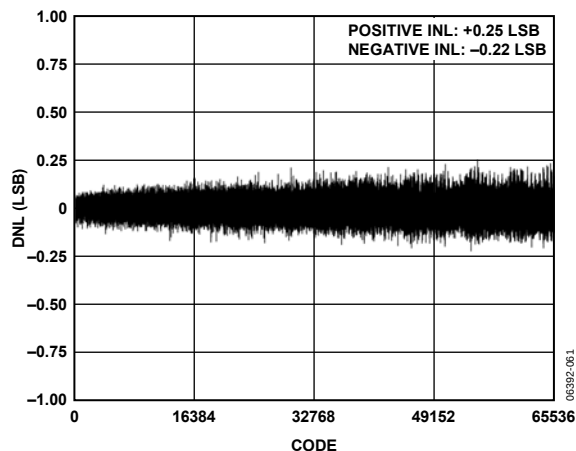
Figure 10. Differential Nonlinearity vs. Code, REF = 2.5 V
