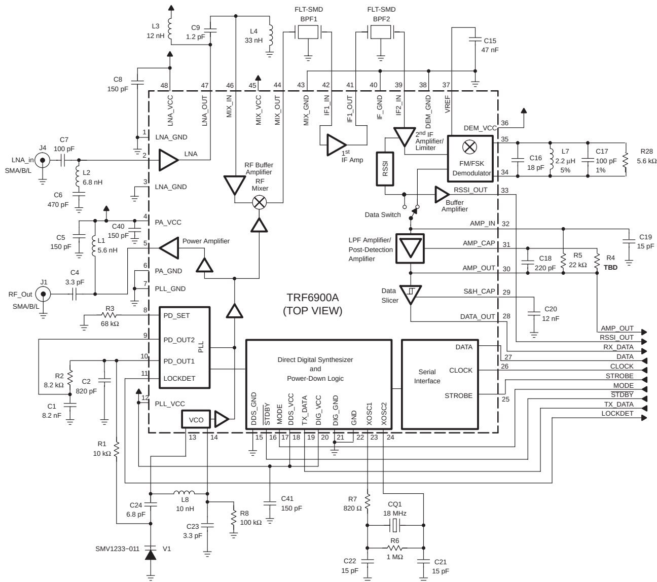
Figure 27. Typical Application Schematic for 868-MHz to 870-MHz European ISM Band
