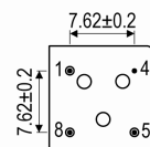
Underside View
