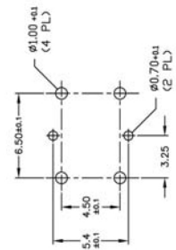
P.C. MOUNTING
