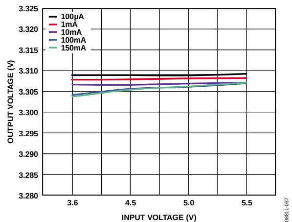
Figure 37. LDO2 Line Regulation Across Output Load, V_{OUT3} = 3.3\text{ V}
