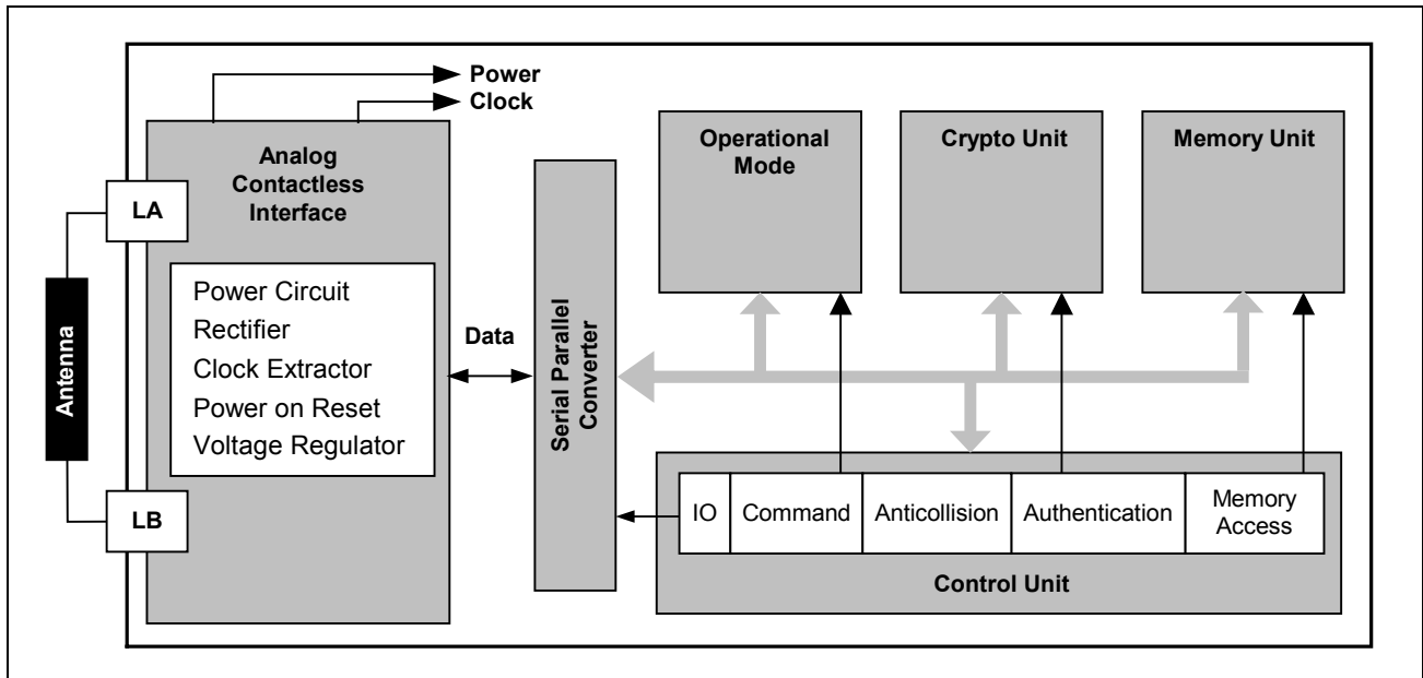
Figure 4 Block diagram of SLE 55R16
