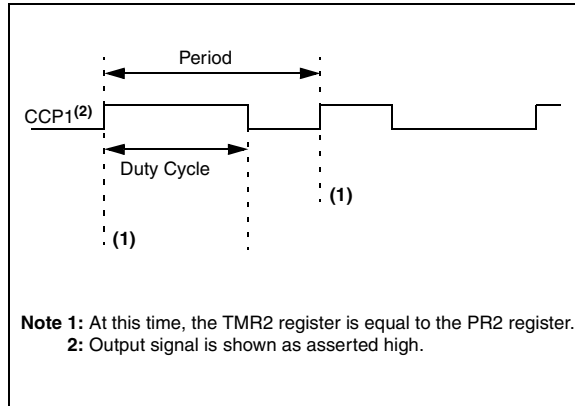
FIGURE 9-4: PWM OUTPUT
