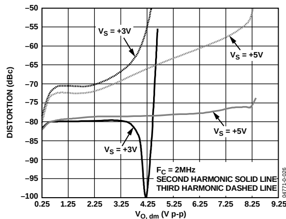
Figure 22. Harmonic Distortion vs. Output Amplitude and Supply, F_C = 2 \text{ MHz}
