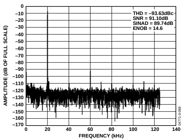
Figure 70. AD8137 Performance on Single 5 V Supply, -1.82 dBFS
