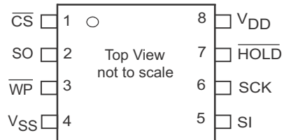
Figure 1. 8-pin SOIC pinout
