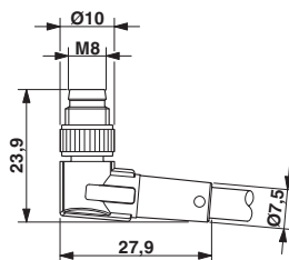
Dimensioned drawing
